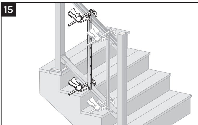
15. Clamp middle vertical(s) in place.
